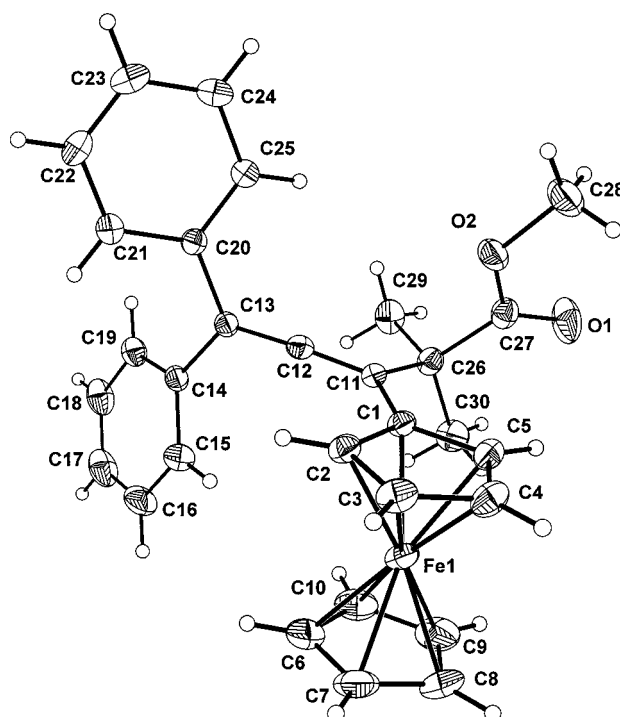
Figure 5. ORTEP plot of 9b ; selected bond lengths [Å], bond angles [°] and torsional angles [°]: C(1)–C(11) 1.482(3), C(11)–C(12) 1.312(3), C(12)–C(13) 1.316(3), C(1)–C(5) 1.431(3), C(4)–C(5) 1.412(3); C(12)–C(11)–C(1) 119.8(2), C(12)–C(11)–C(26) 119.9(2), C(11)–C(12)–C(13) 175.0(2); C(11)–C(1)–C(2)–C(3) 175.2(2), C(2)–C(1)–C(11)–C(12) 4.1(3), C(2)–C(1)–C(11)–C(26) 176.9(2)
