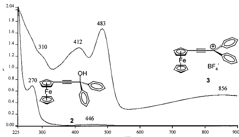
Figure 4. UV/Vis spectra of 2 (λ max at 270 and 446 nm) and 3 (λ max at 310sh, 412, 483, and 856 nm) at –70 °C (dichloromethane)
