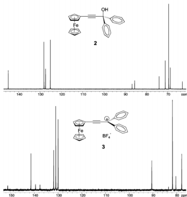
Figure 2. ^{13}\text{C} -NMR spectra of 2 (top) and 3 (bottom) ( -70^\circ\text{C} , \text{CD}_2\text{Cl}_2 , 100 MHz)
