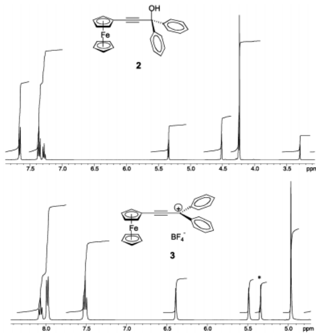
Figure 2. ^1\text{H} -NMR spectra ( -70^\circ\text{C} , \text{CD}_2\text{Cl}_2 , 400 MHz) of 2 (top) and 3 (bottom)
