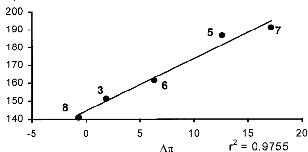
Figure 3. Correlation of the Δ π values (Δ π = δ para – δ meta ) and the C γ resonance (carbenium or quaternary benzyl center) of the propargyl cations 3 , 5 , 6 , and the resonance compounds 7 and 8
